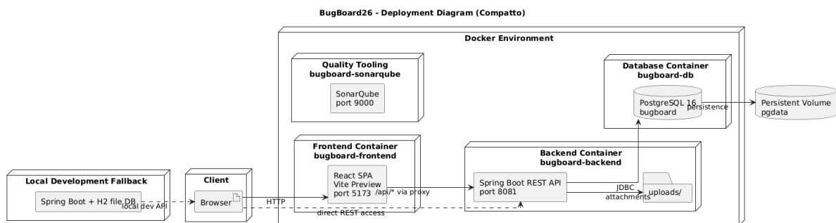
Figura 17: Deployment Diagram — BugBoard26
